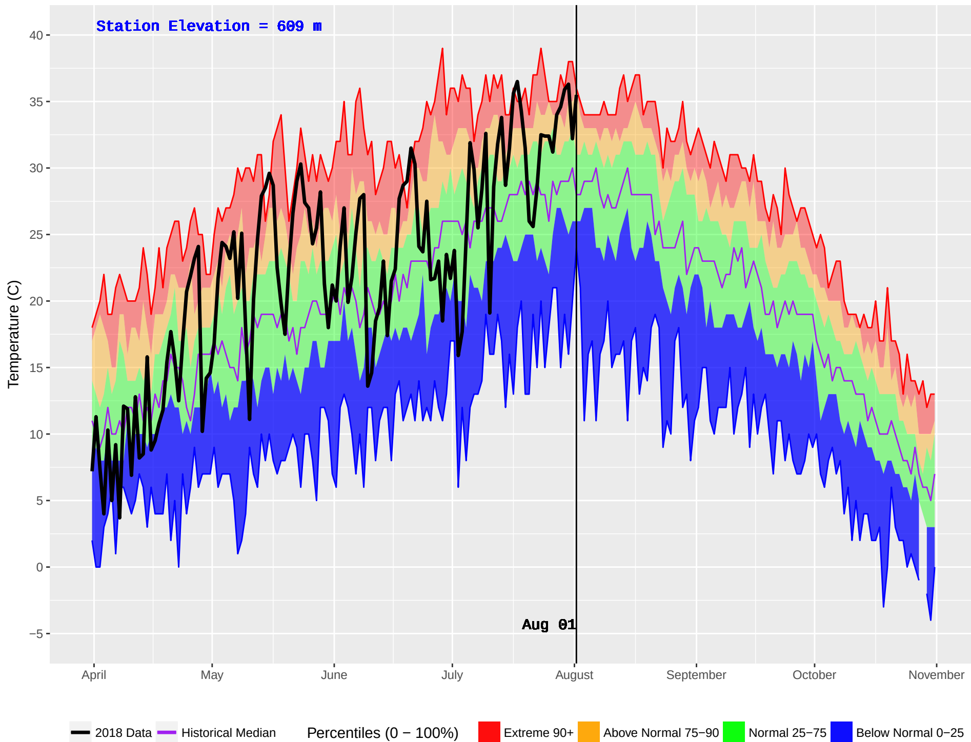
ROCK CREEK (394) : Historical (1990–2016) and Current (2018) Daily Temperature
